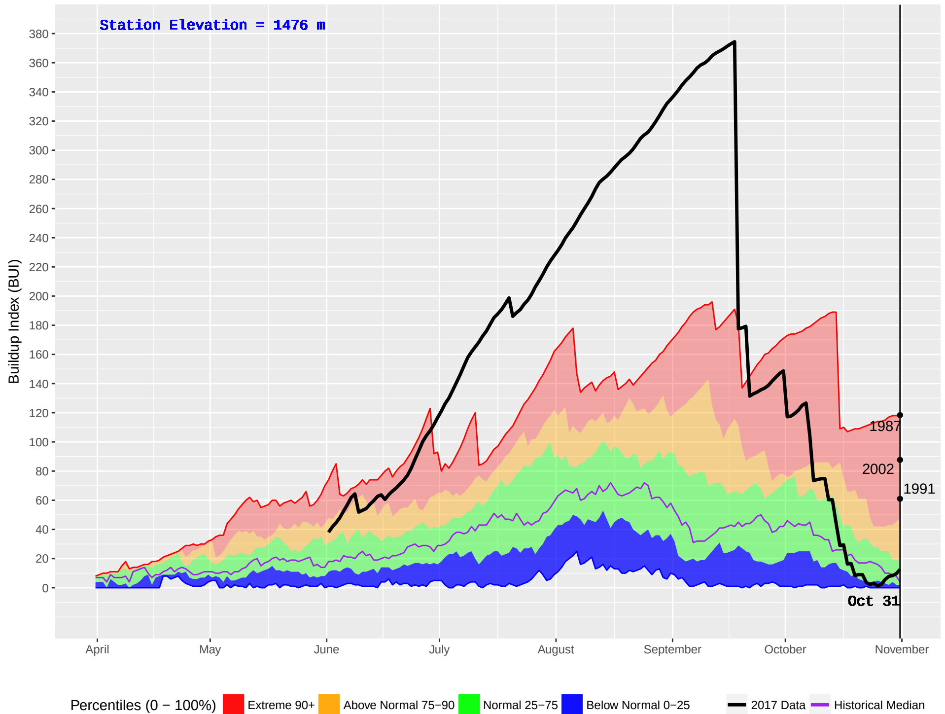
BRENDA MINES (283) : Historical (1977–2016) and Current (2017) Noon Buildup Index (BUI)
